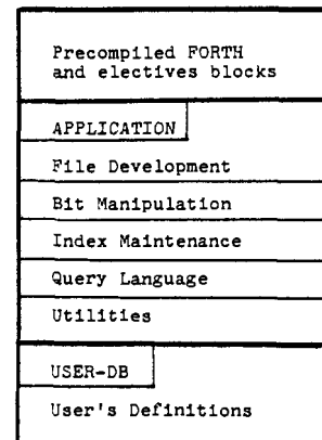
Figure 2. Dictionary Layout
