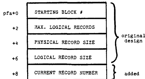
Figure 1. File Information Block
