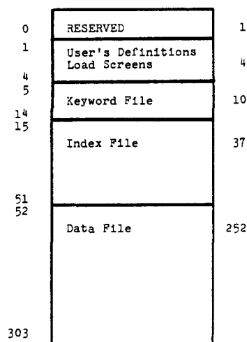
Figure 4. Example Diskette Allocation
