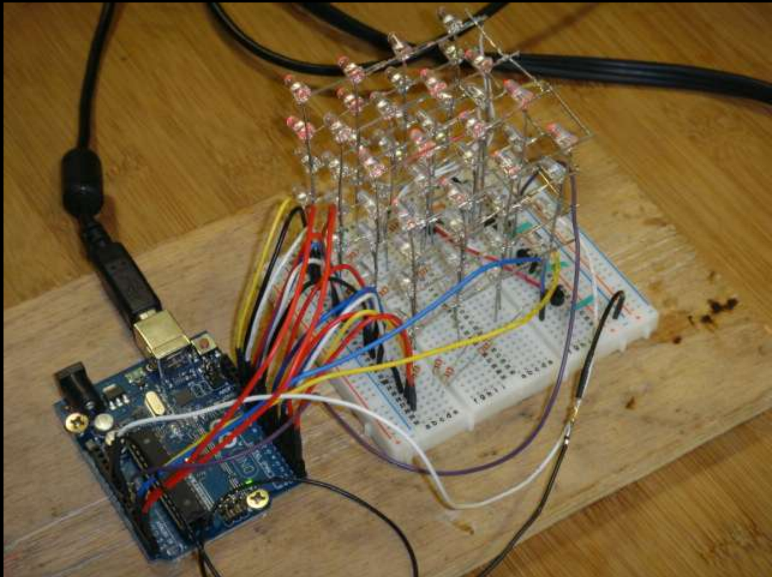
Ting's 4x4x4 LED cube powered by an Arduino & Forth
